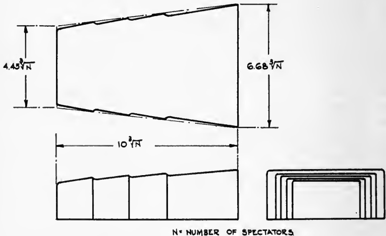
FIG. 2. Elevation and plan of auditorium without balcony.
